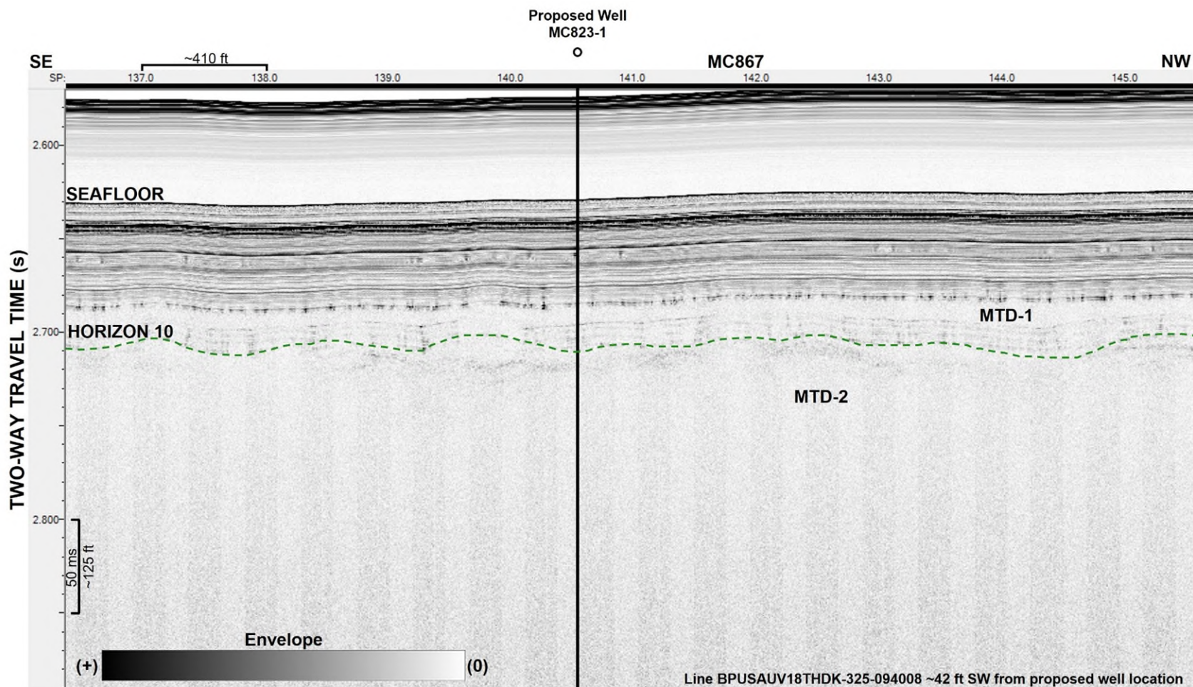
Figure 6. SBP Line BPUSAUV18THDK -325-094008 showing high resolution shallow stratigraphy at Proposed Well MC823-1 (MTD= Mass Transport Deposits).
