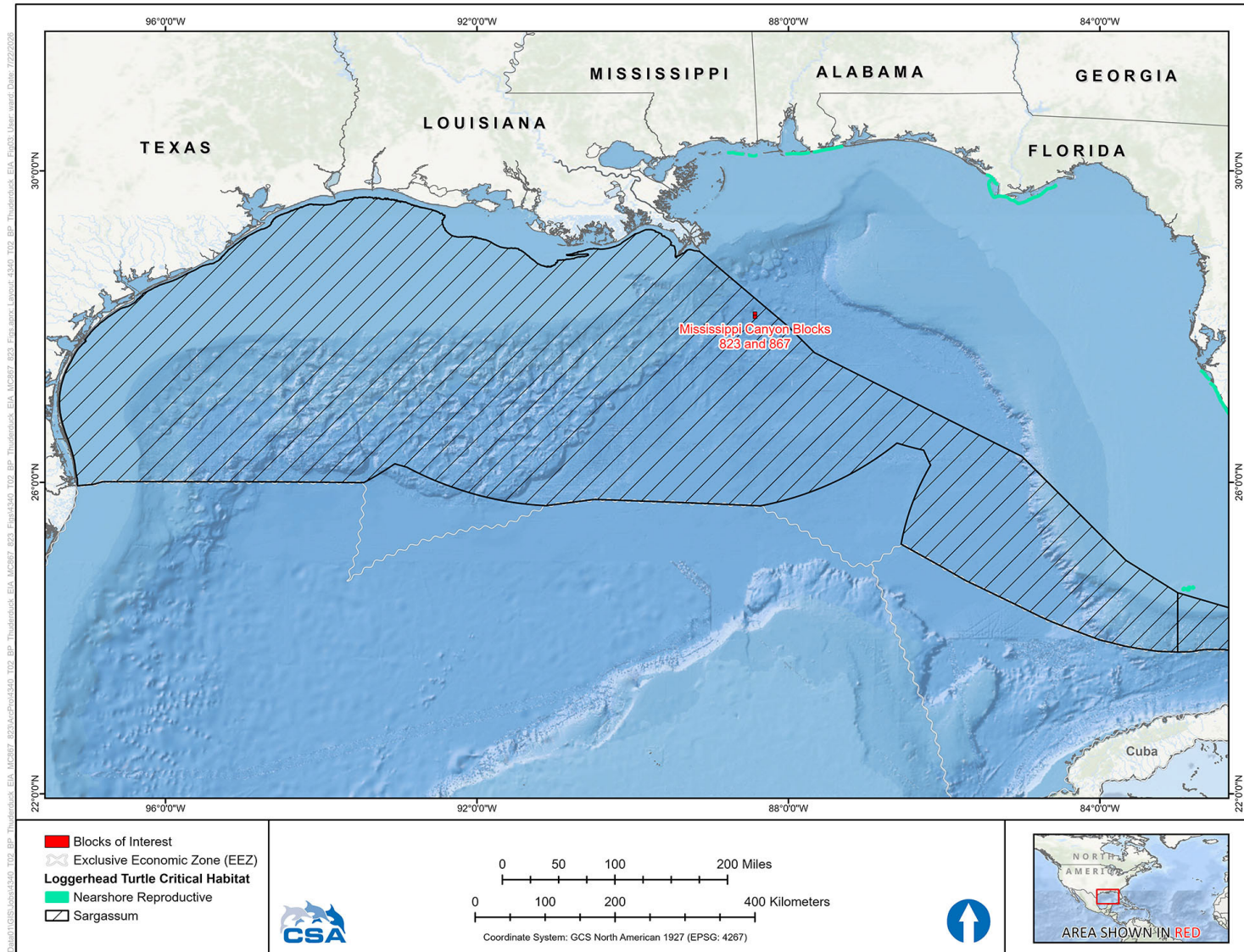
Figure 4. Location of loggerhead turtle designated Sargassum critical habitat and nearshore reproductive critical habitat in relation to the project area.
