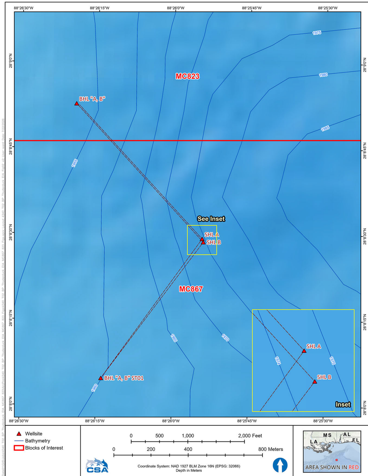
Figure 2. Bathymetric map of the project area showing in the location of the proposed primary and backup wells in Mississippi Canyon Blocks 867 and 823.
