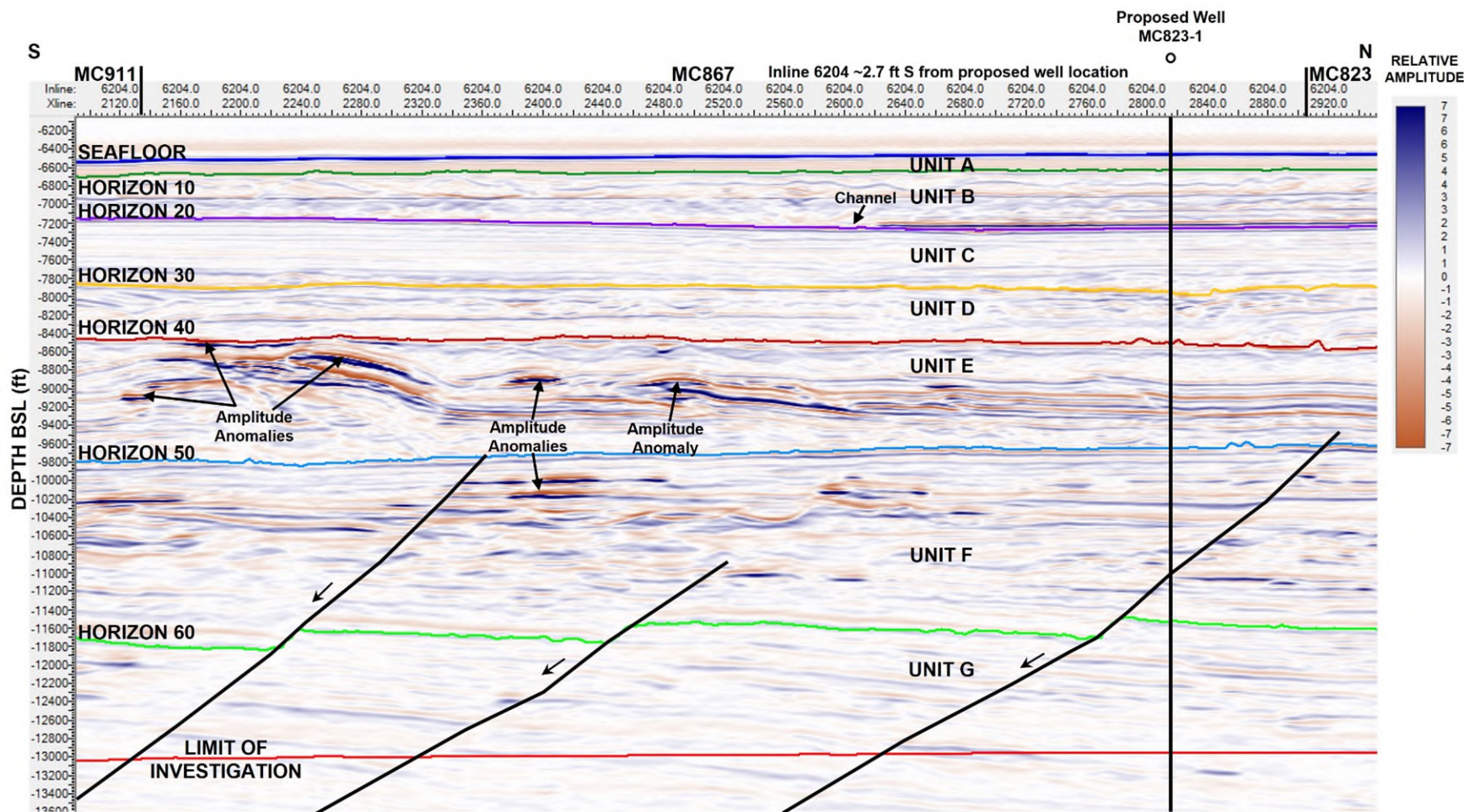
Figure 7. 3D seismic Inline 6204 through Proposed Well MC823-1 showing mapped stratigraphic horizons, faulting, presence of amplitude anomalies, and unit stratigraphy associated with this report. Direction of downdip fault motion shown by arrows (BSL= Below Sea Level).
