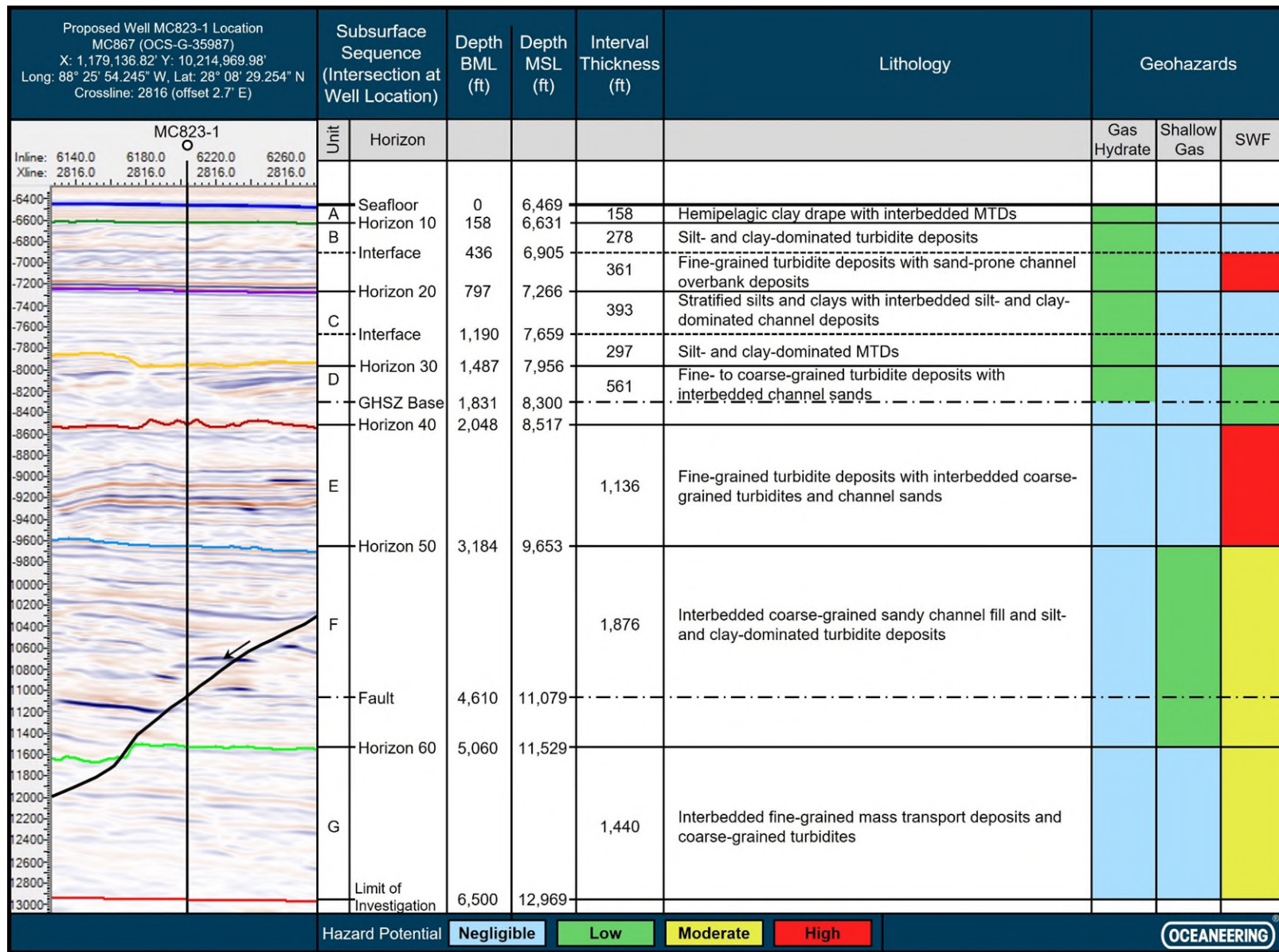
Figure 9. Top-Hole Prognosis for Proposed Well MC823-1.
