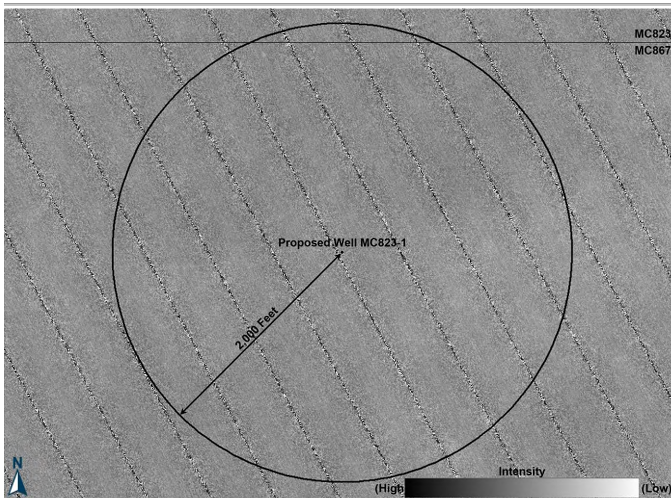
Figure 2. Multibeam Backscatter displaying low intensity within 2,000 ft of Proposed Well MC823-1.
