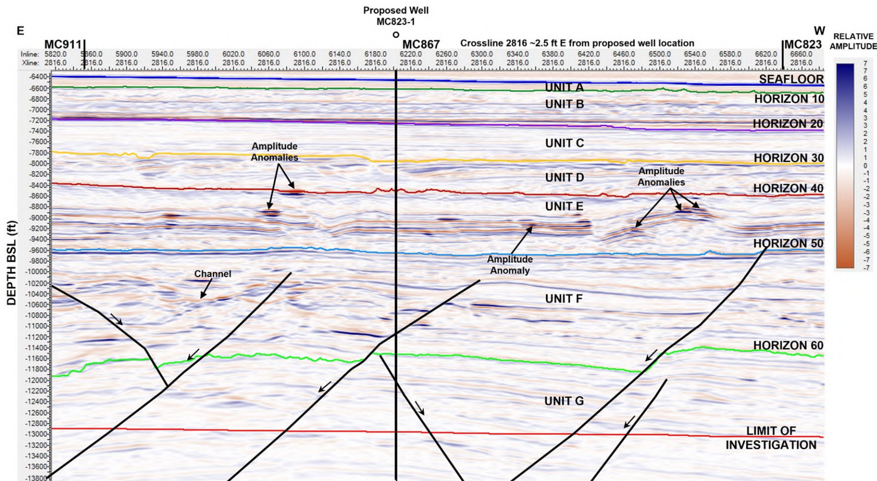
Figure 8. 3D seismic Crossline 2816 through Proposed Well MC823-1 showing mapped stratigraphic horizons, faulting, presence of amplitude anomalies, and unit stratigraphy associated with this report. Direction of down-dip fault motion shown by arrows (BSL= Below Sea Level).
