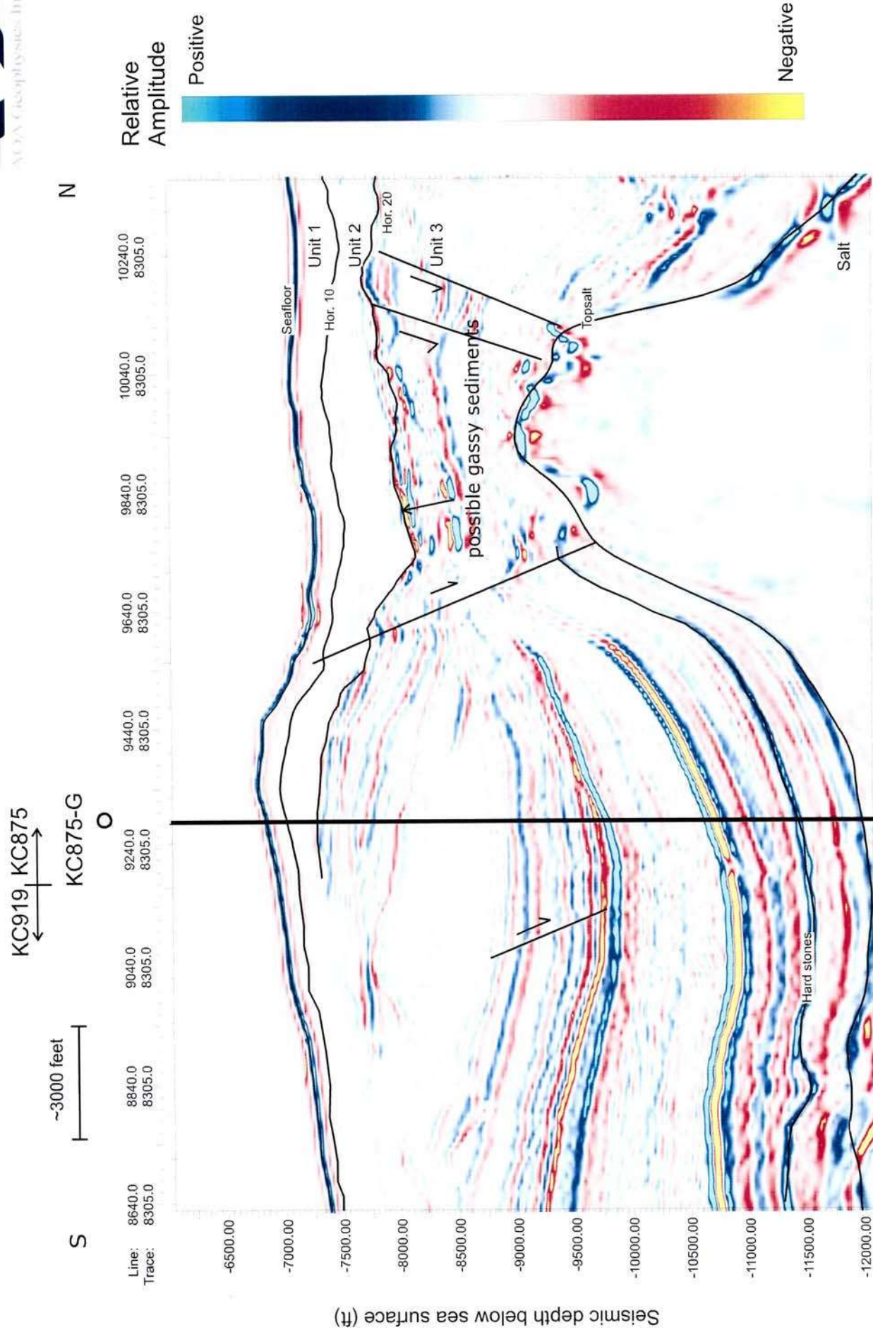
3-D reprocessed Seismic Record, crossline 8305, Location G Block 875, Keathley Canyon Area
