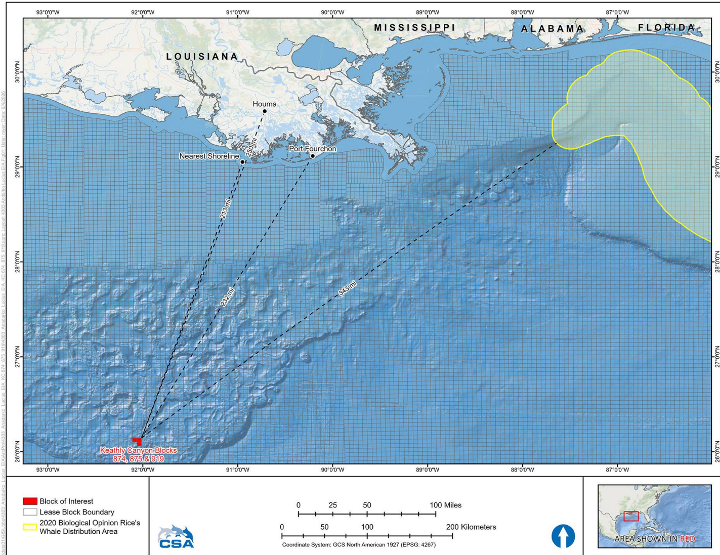
Figure 1. Location of Keathley Canyon Blocks 874, 875, and 919 relative to the Louisiana shoreline, the Rice's whale habitat area, and offshore bathymetric contours.
