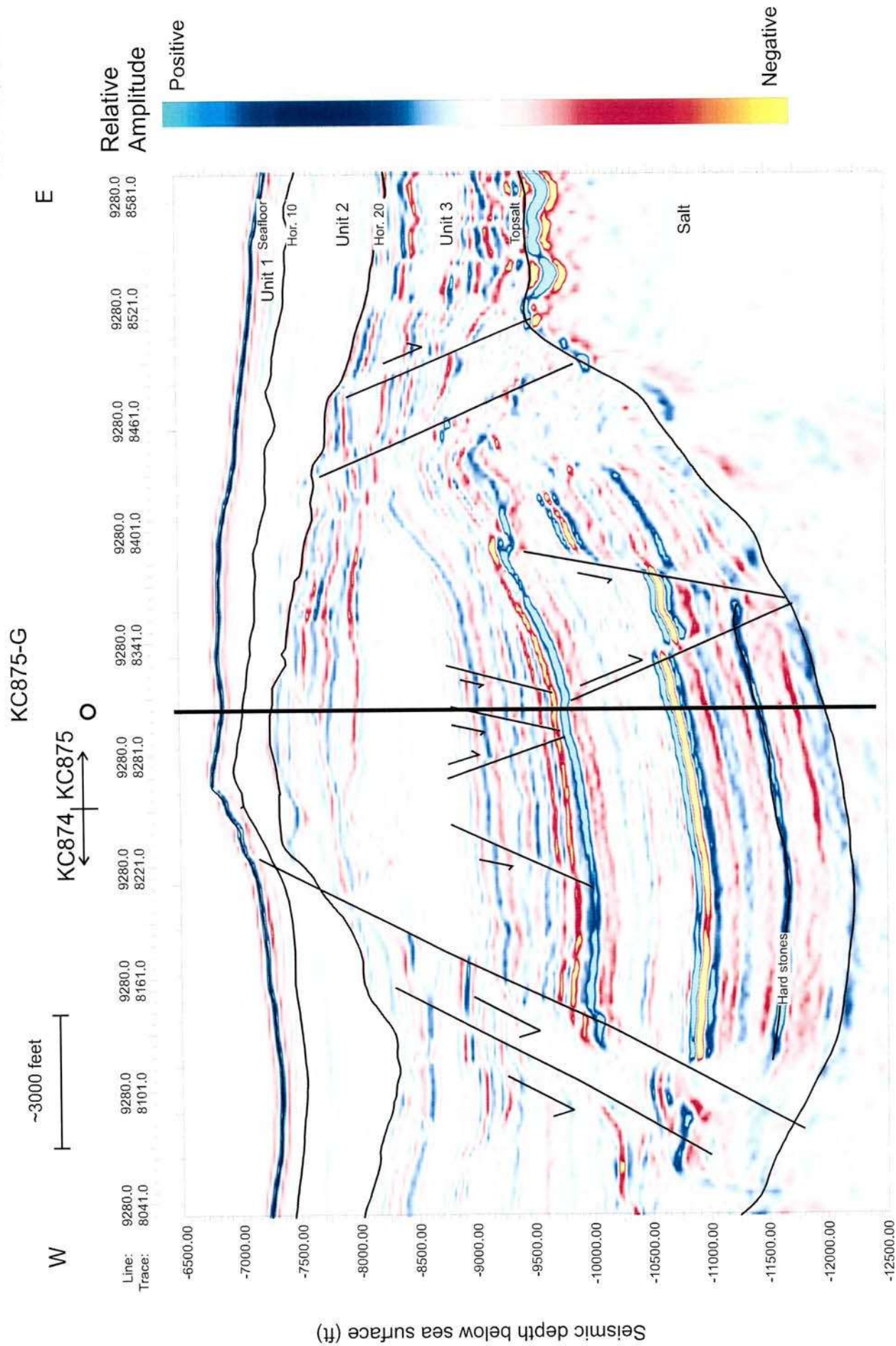
3-D reprocessed Seismic Record, inline 9280, Location G Block 875, Keathley Canyon Area
