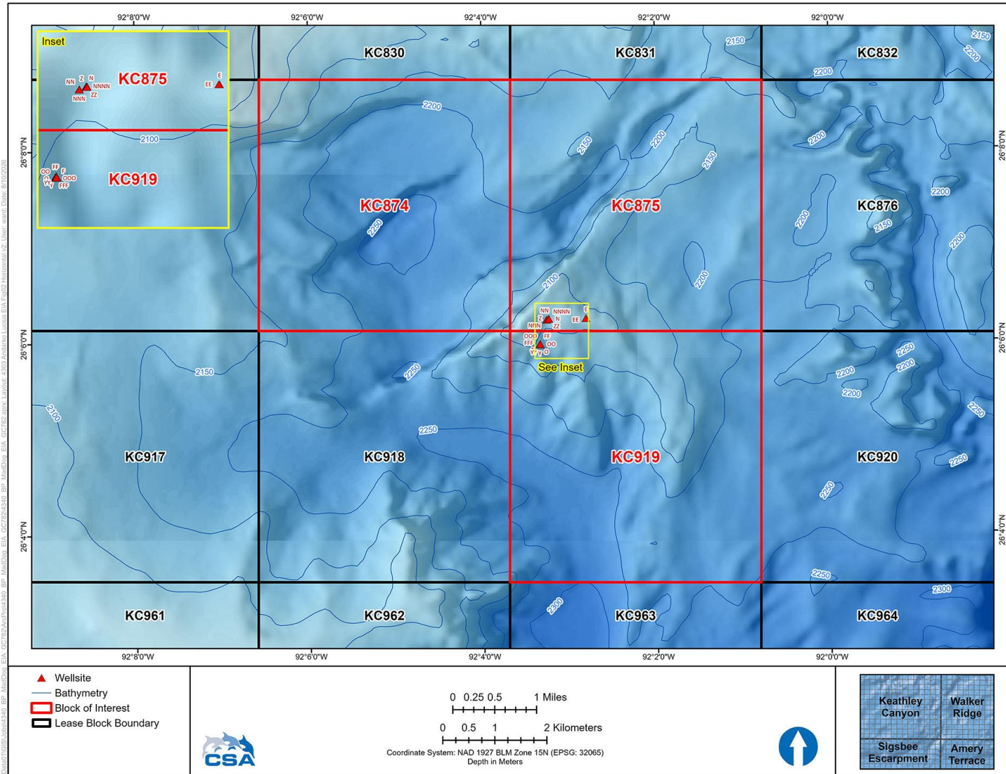
Figure 2. Bathymetric map of the project area showing the surface hole location of the wellsites in Keathley Canyon Blocks 875 and 919.
