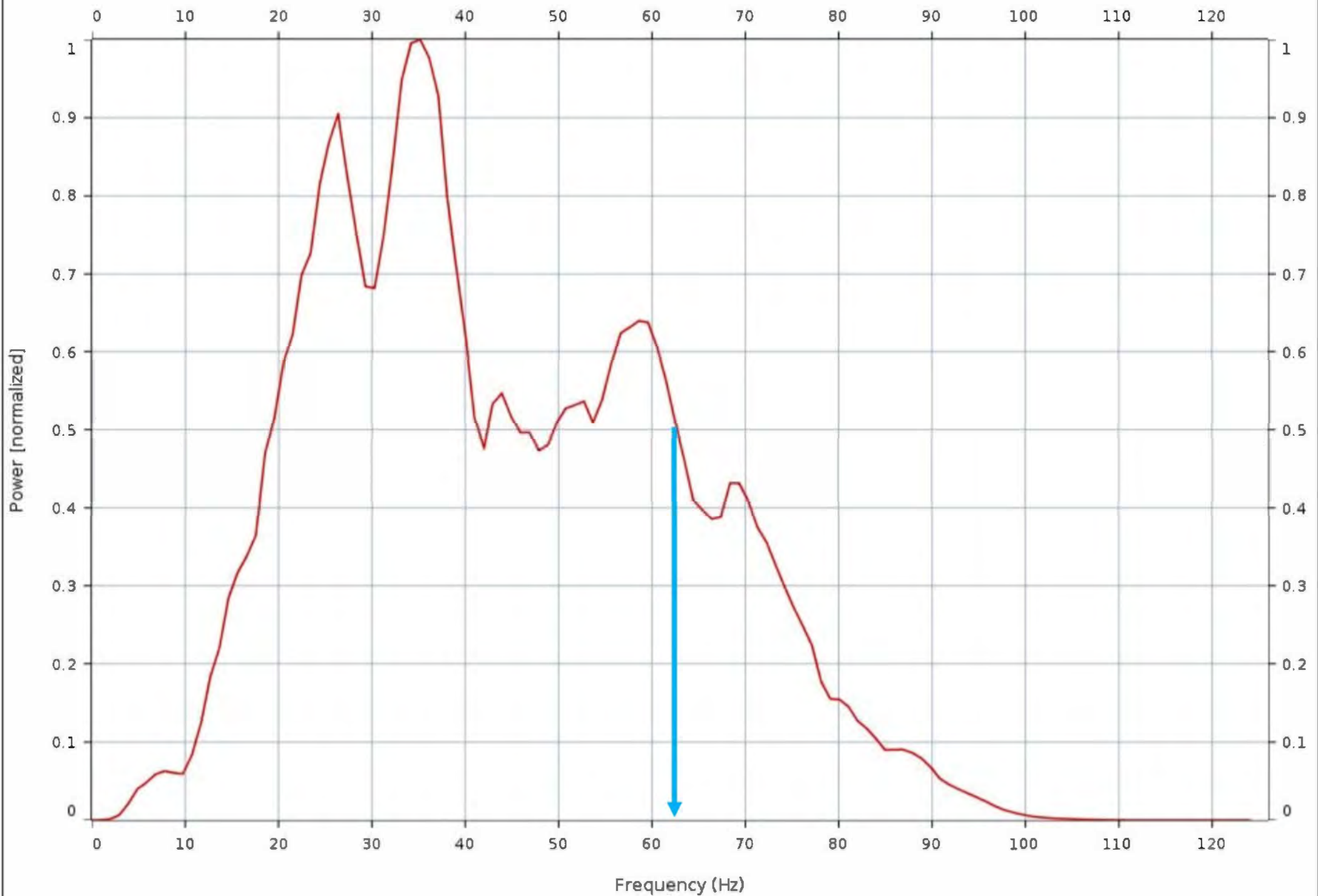
Frequency Spectrum - Proposed Well A
